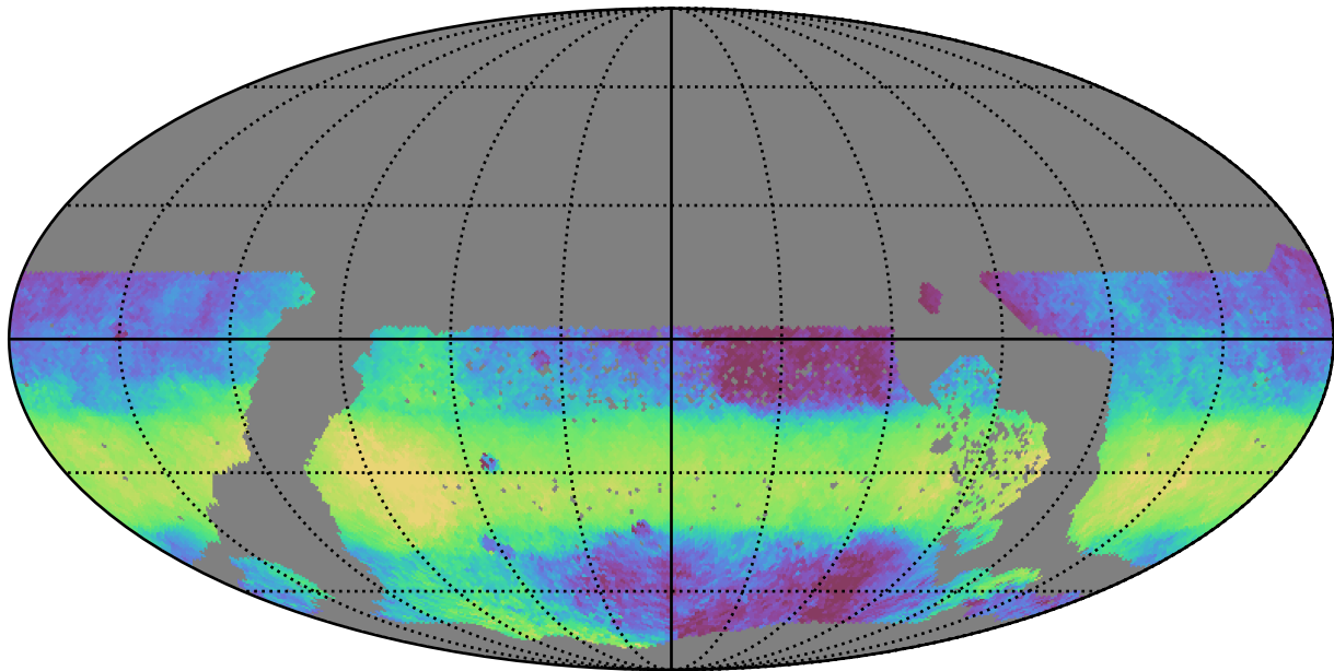
too_elab_r16_d2_griz_v3.4_10yrs WFD y band: Median HA
