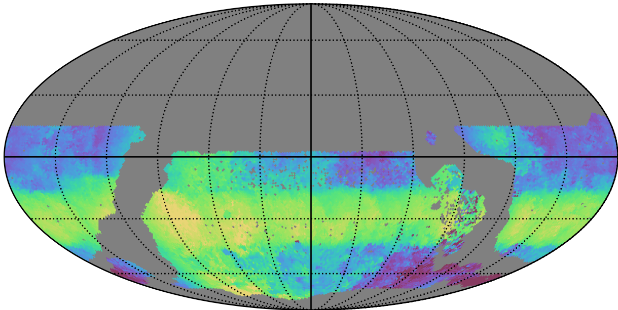
too_elab_r16_d2_griz_v3.4_10yrs WFD u band: Median HA
