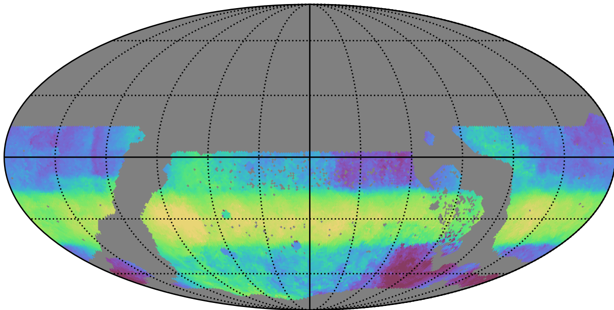
too_elab_r16_d2_griz_v3.4_10yrs WFD r band: Median HA
