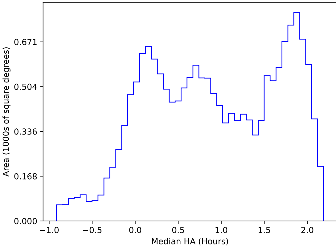
too_elab_r16_d2_griz_v3.4_10yrs WFD r band: Median HA
