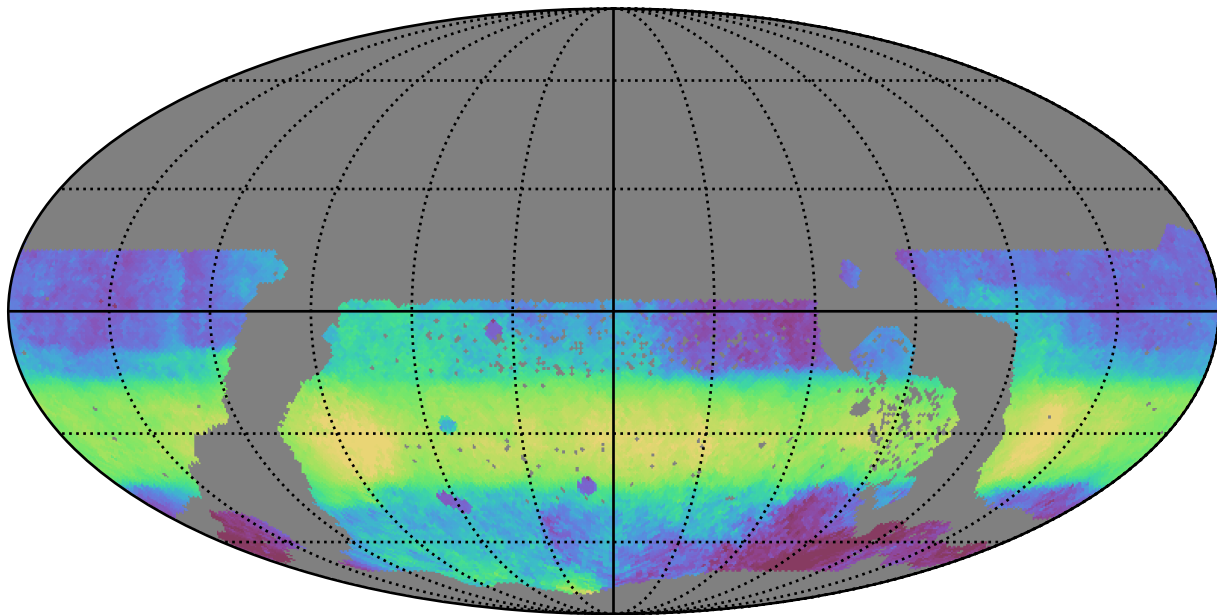
too_elab_r16_d2_griz_v3.4_10yrs WFD i band: Median HA
