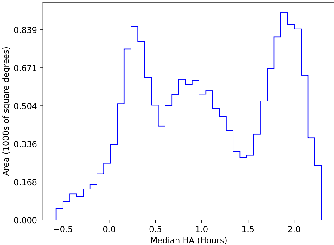
too_elab_r16_d2_griz_v3.4_10yrs WFD i band: Median HA
