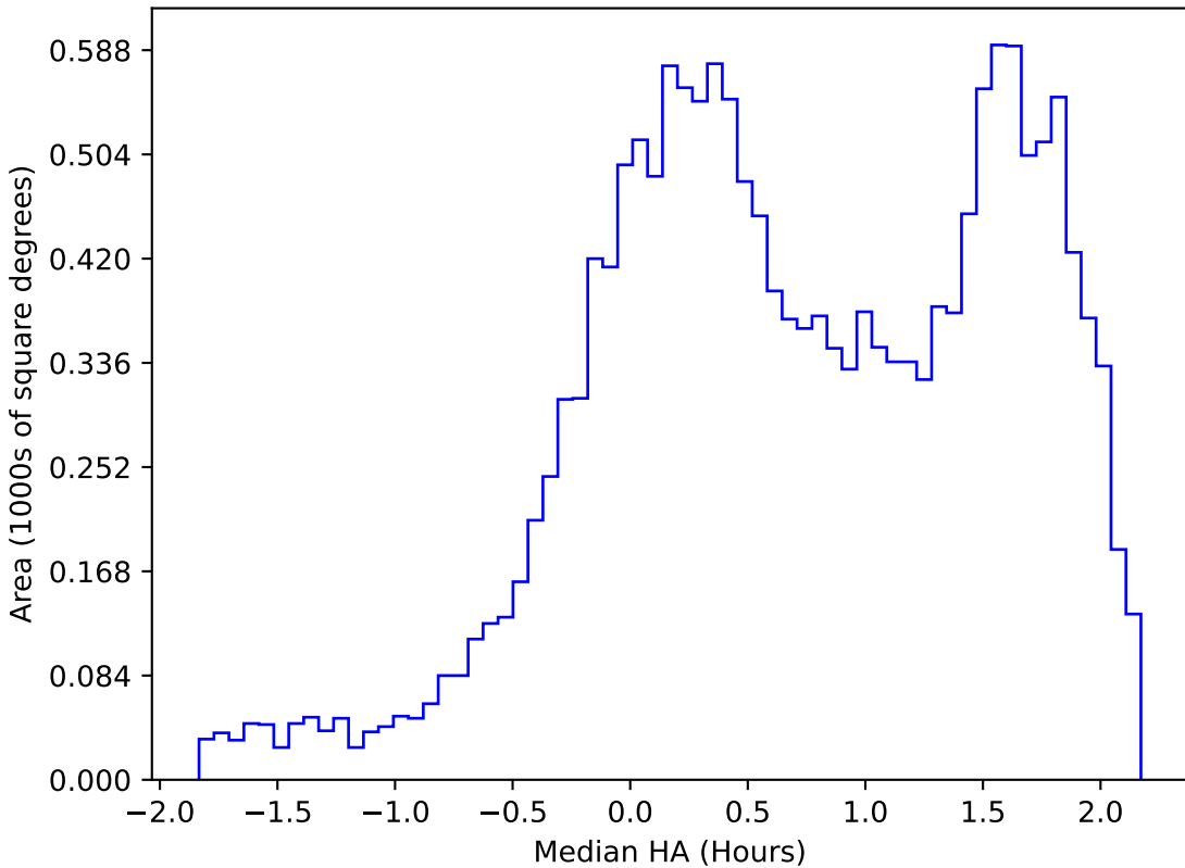
too_elab_r16_d2_griz_v3.4_10yrs WFD g band: Median HA
