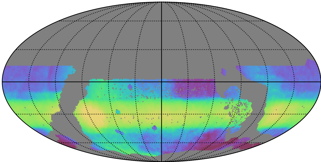
too_elab_r16_d2_griz_v3.4_10yrs WFD all bands: Median HA
