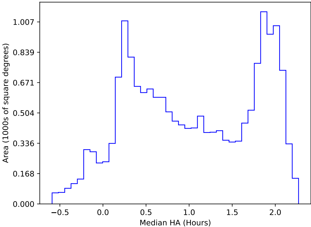
too_elab_r16_d2_griz_v3.4_10yrs WFD all bands: Median HA
