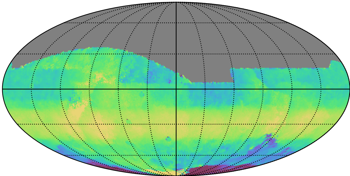
too_elab_r16_d2_griz_v3.4_10yrs All sky z band: Median HA
