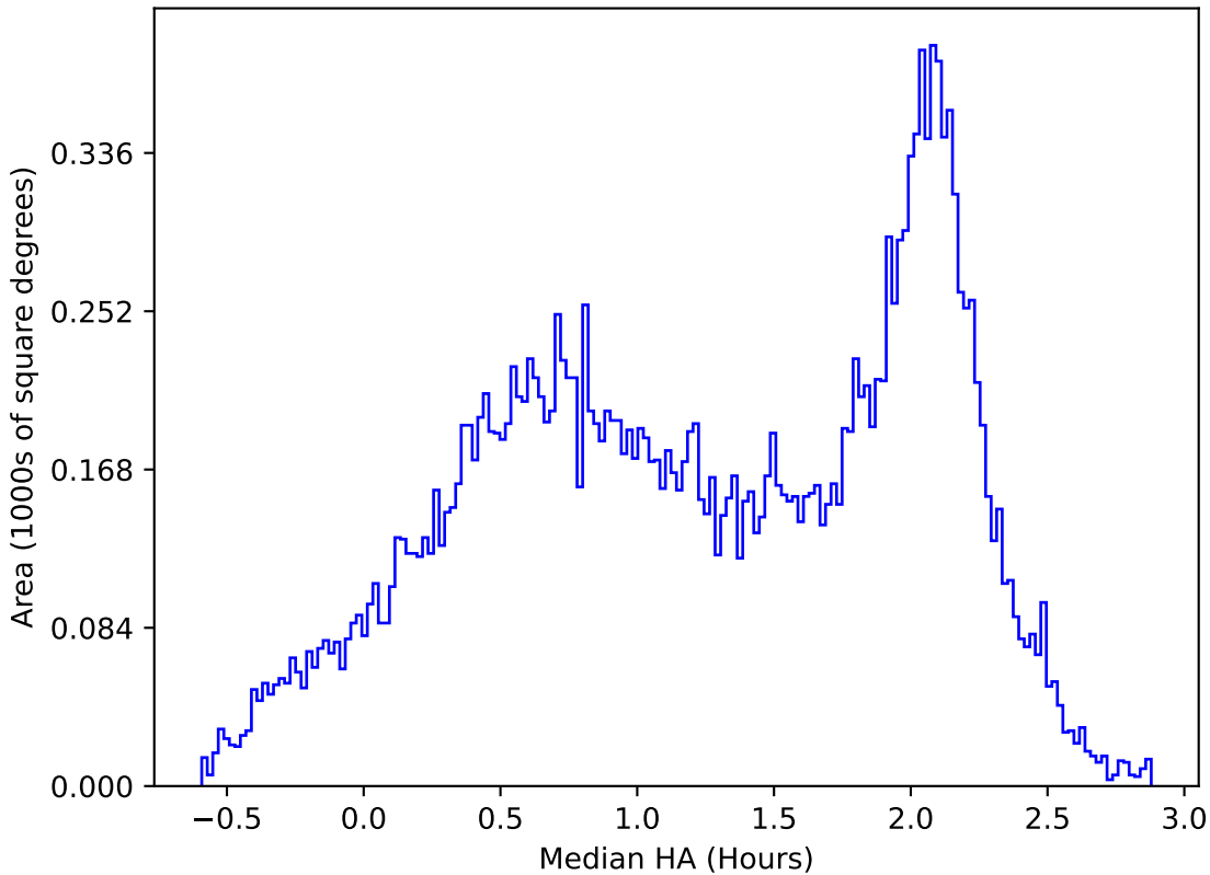
too_elab_r16_d2_griz_v3.4_10yrs All sky y band: Median HA
