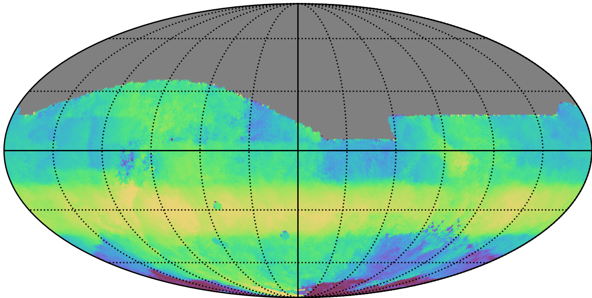
too_elab_r16_d2_griz_v3.4_10yrs All sky r band: Median HA
