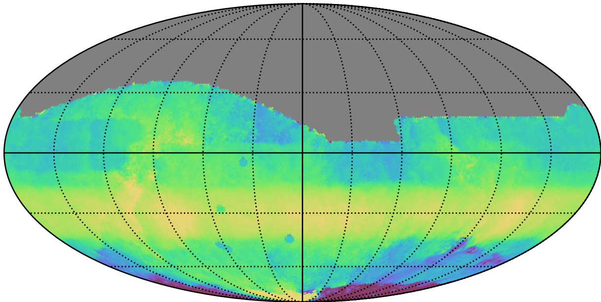
too_elab_r16_d2_griz_v3.4_10yrs All sky i band: Median HA
