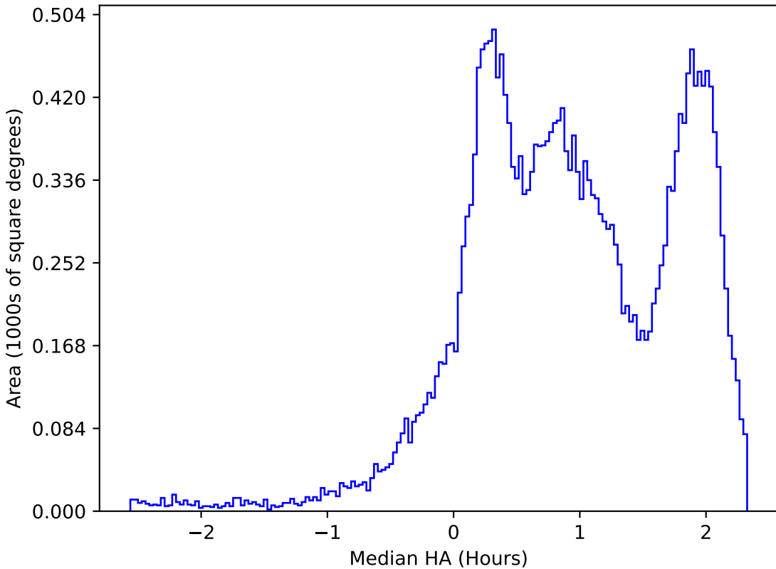
too_elab_r16_d2_griz_v3.4_10yrs All sky i band: Median HA
