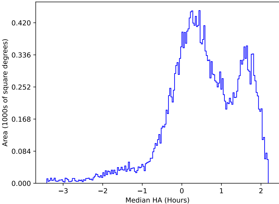
too_elab_r16_d2_griz_v3.4_10yrs All sky g band: Median HA
