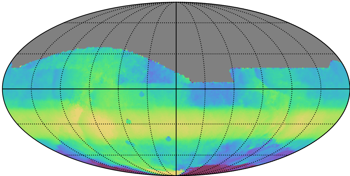
too_elab_r16_d2_griz_v3.4_10yrs All sky all bands: Median HA
