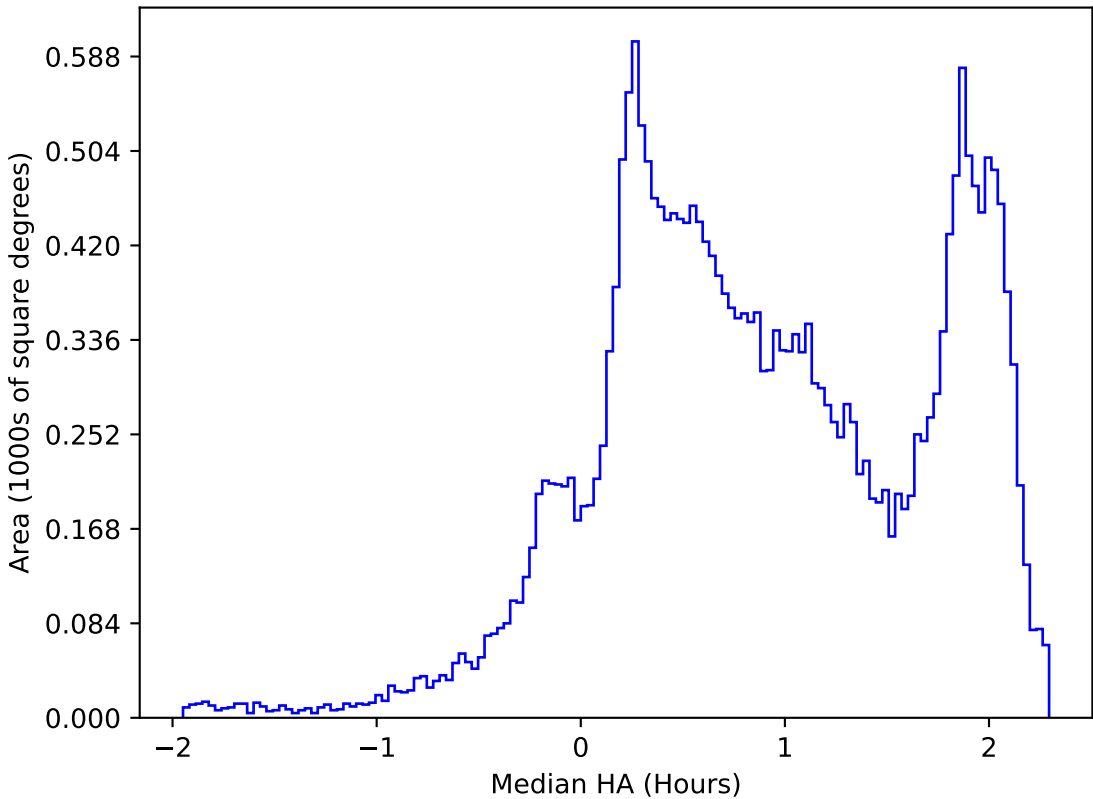
too_elab_r16_d2_griz_v3.4_10yrs All sky all bands: Median HA
