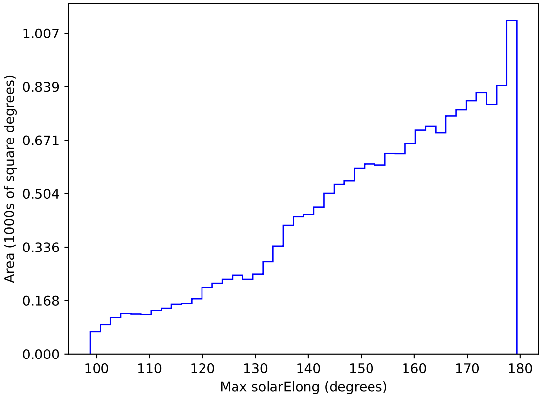
too_elab_r16_d2_griz_v3.4_10yrs WFD z band: Max solarElong
