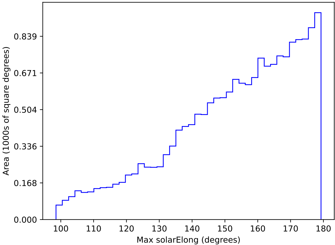
too_elab_r16_d2_griz_v3.4_10yrs WFD y band: Max solarElong
