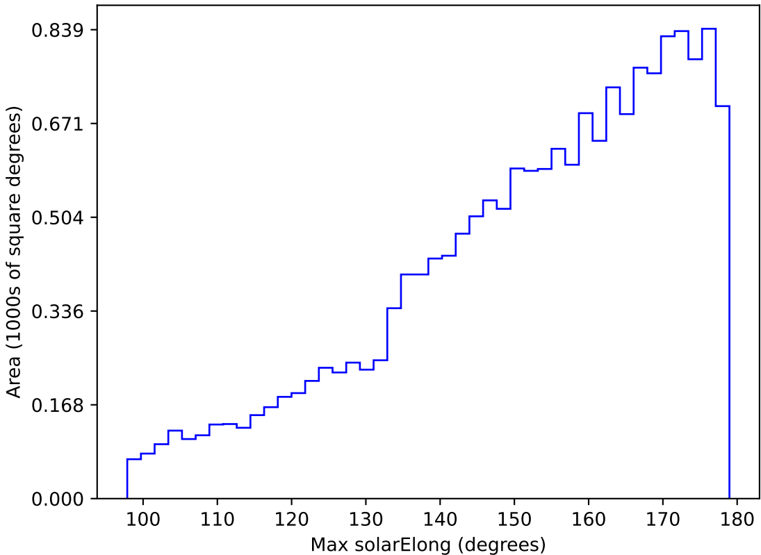
too_elab_r16_d2_griz_v3.4_10yrs WFD u band: Max solarElong
