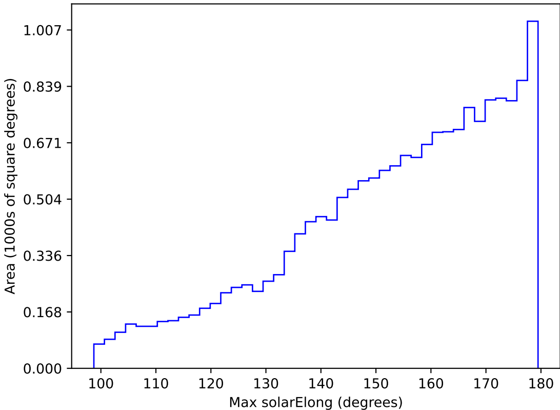
too_elab_r16_d2_griz_v3.4_10yrs WFD r band: Max solarElong
