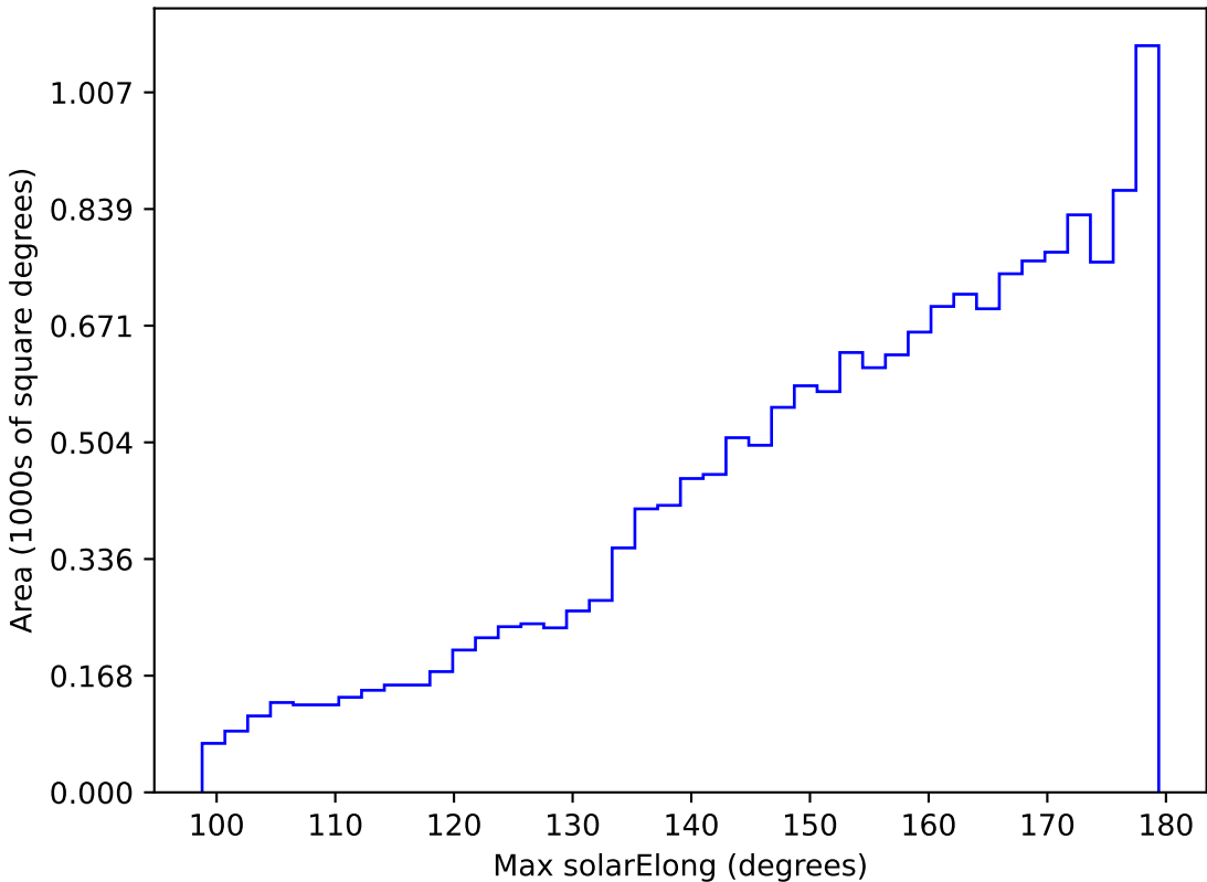
too_elab_r16_d2_griz_v3.4_10yrs WFD i band: Max solarElong
