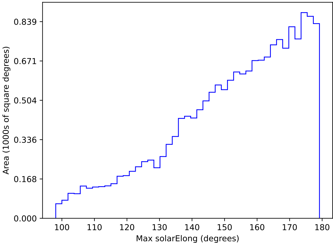
too_elab_r16_d2_griz_v3.4_10yrs WFD g band: Max solarElong
