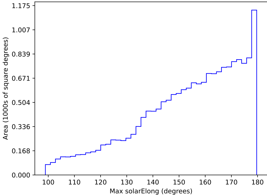
too_elab_r16_d2_griz_v3.4_10yrs WFD all bands: Max solarElong
