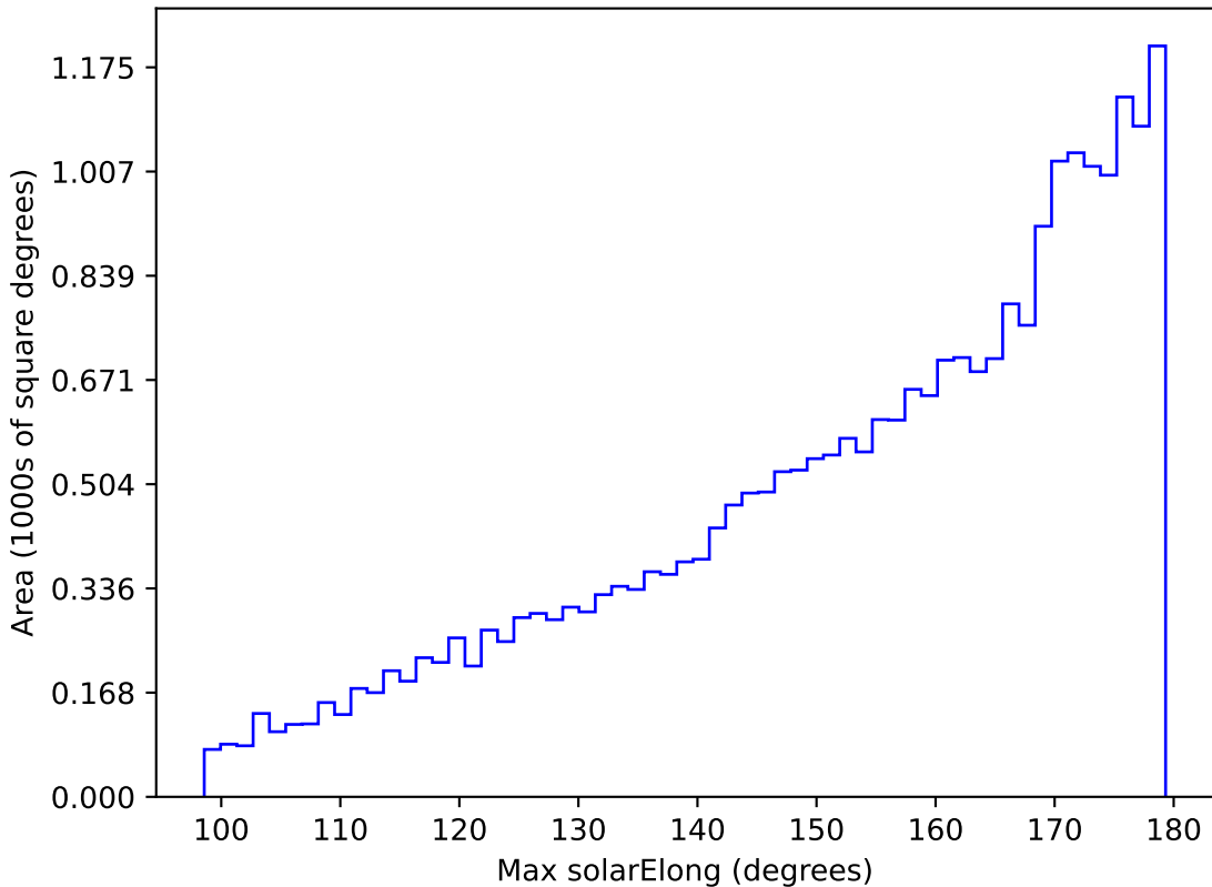
too_elab_r16_d2_griz_v3.4_10yrs All sky z band: Max solarElong
