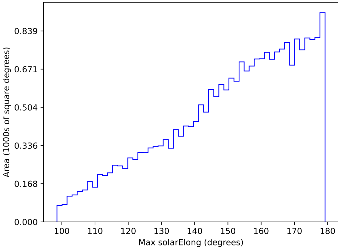
too_elab_r16_d2_griz_v3.4_10yrs All sky y band: Max solarElong
