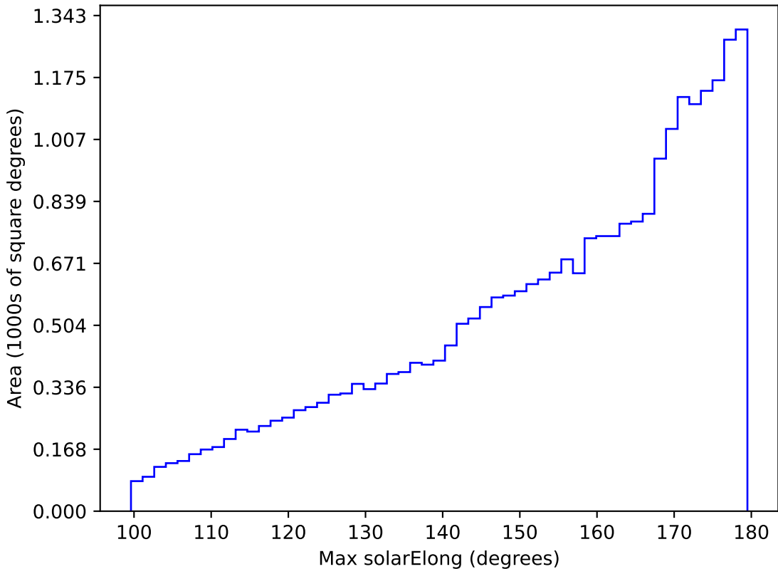
too_elab_r16_d2_griz_v3.4_10yrs All sky r band: Max solarElong
