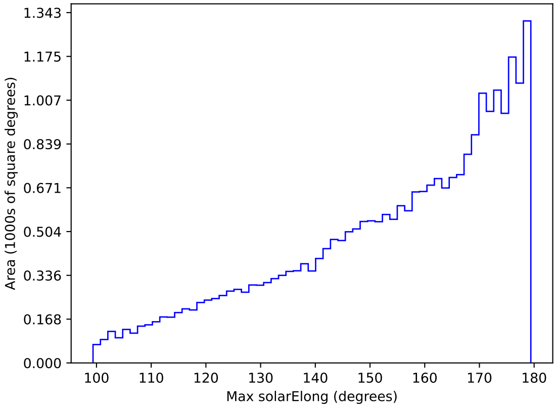
too_elab_r16_d2_griz_v3.4_10yrs All sky i band: Max solarElong
