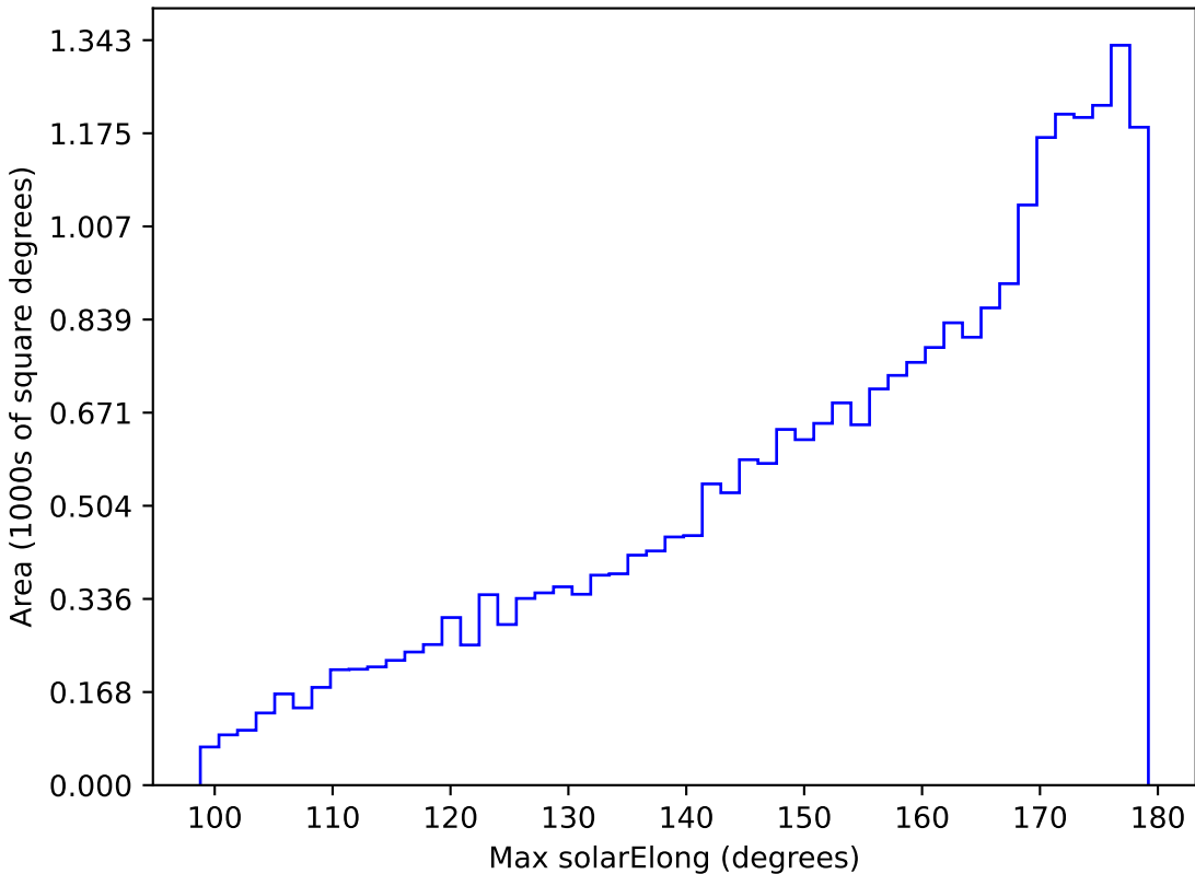
too_elab_r16_d2_griz_v3.4_10yrs All sky g band: Max solarElong
