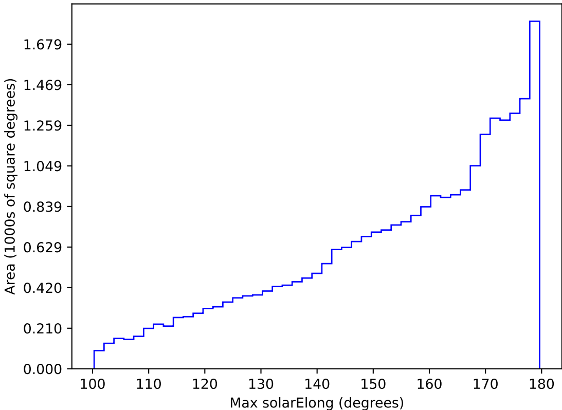
too_elab_r16_d2_griz_v3.4_10yrs All sky all bands: Max solarElong
