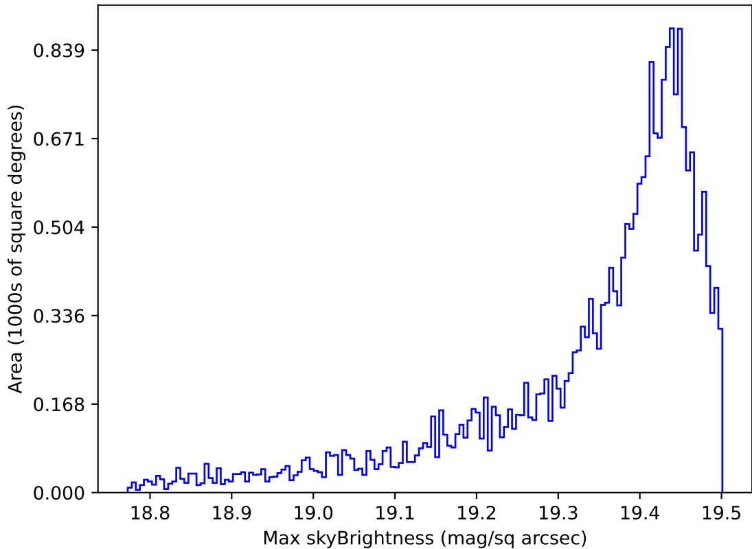
too_elab_r16_d2_griz_v3.4_10yrs Yr 1 z band: Max skyBrightness
