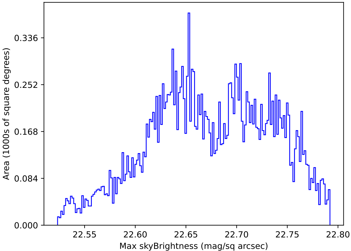
too_elab_r16_d2_griz_v3.4_10yrs Yr 1 u band: Max skyBrightness
