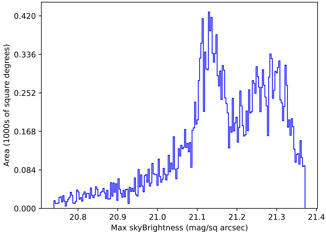
too_elab_r16_d2_griz_v3.4_10yrs Yr 1 r band: Max skyBrightness
