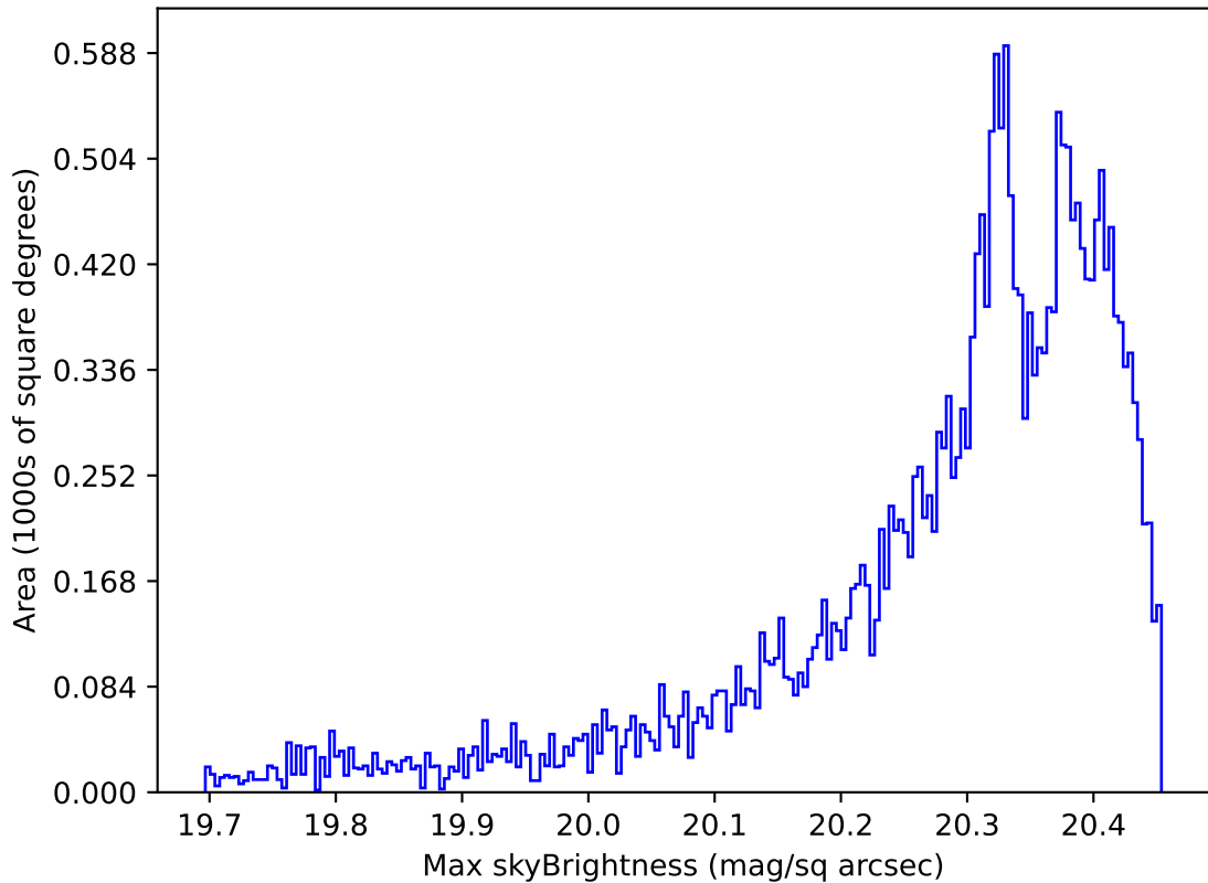
too_elab_r16_d2_griz_v3.4_10yrs Yr 1 i band: Max skyBrightness
