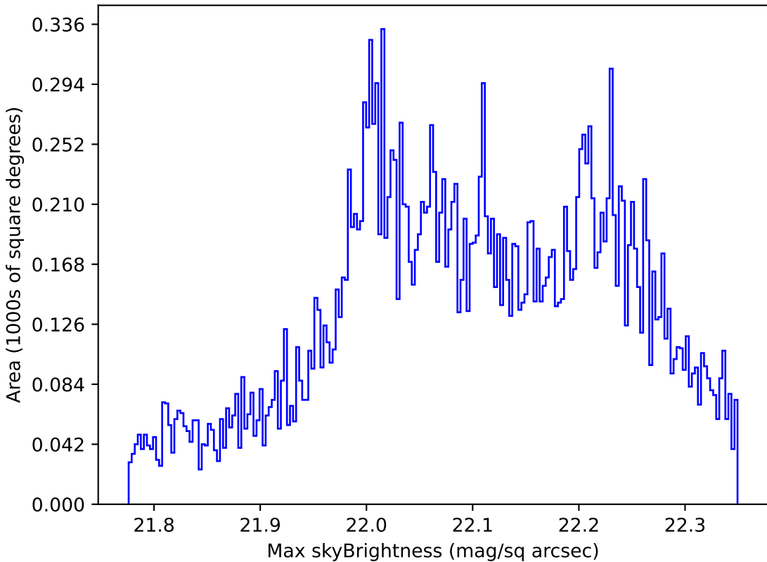
too_elab_r16_d2_griz_v3.4_10yrs Yr 1 g band: Max skyBrightness
