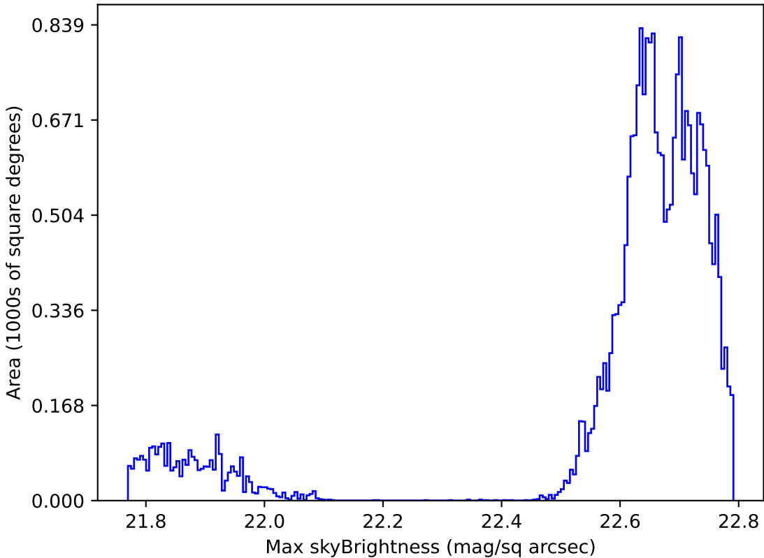
too_elab_r16_d2_griz_v3.4_10yrs Yr 1 all bands: Max skyBrightness
