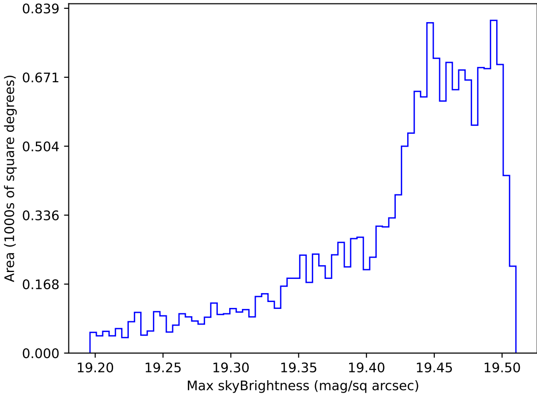
too_elab_r16_d2_griz_v3.4_10yrs WFD z band: Max skyBrightness
