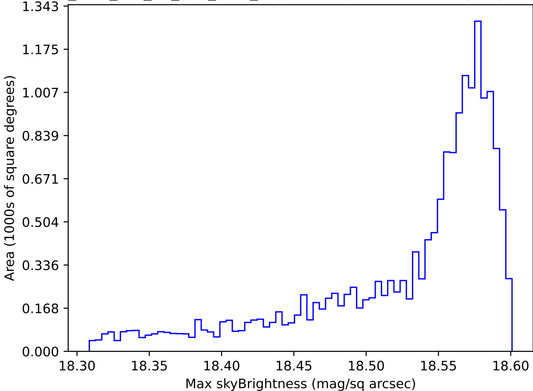
too_elab_r16_d2_griz_v3.4_10yrs WFD y band: Max skyBrightness
