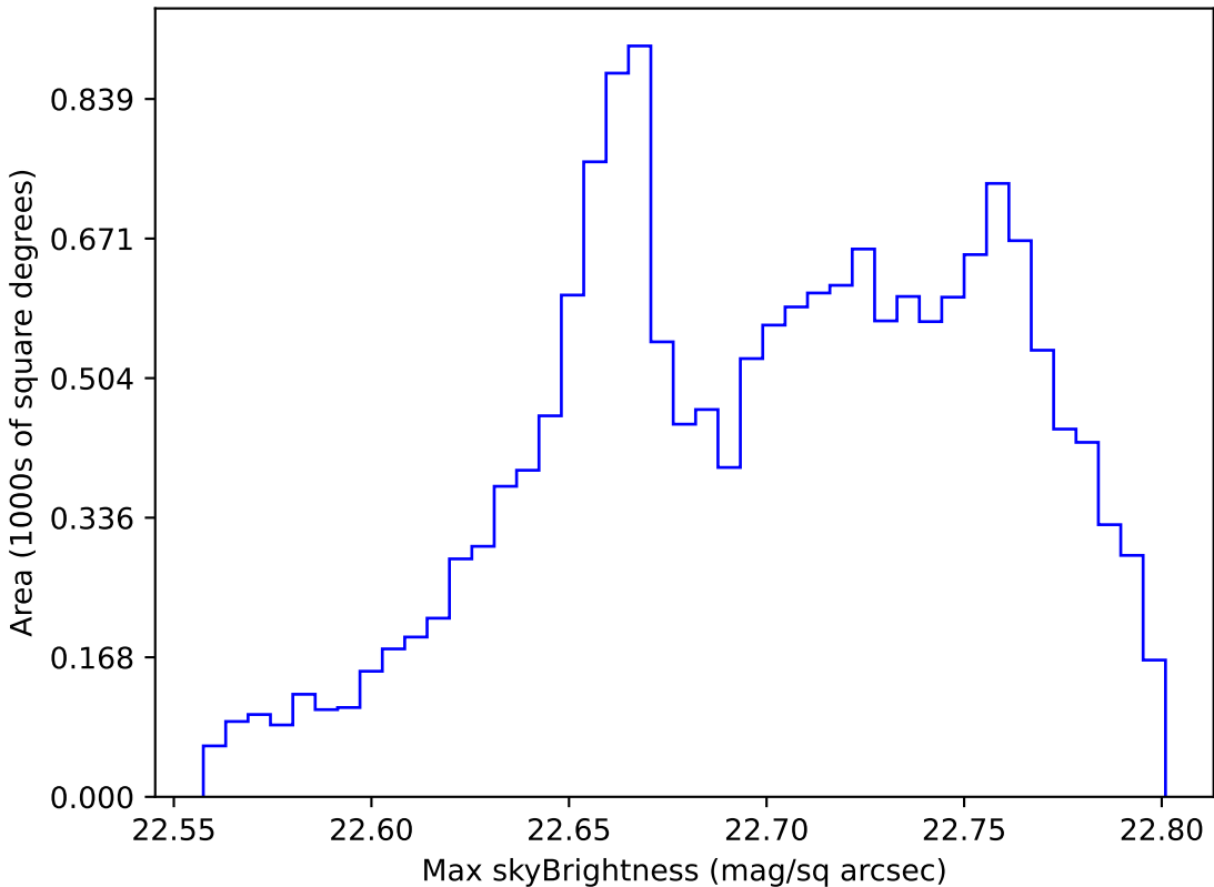
too_elab_r16_d2_griz_v3.4_10yrs WFD u band: Max skyBrightness
