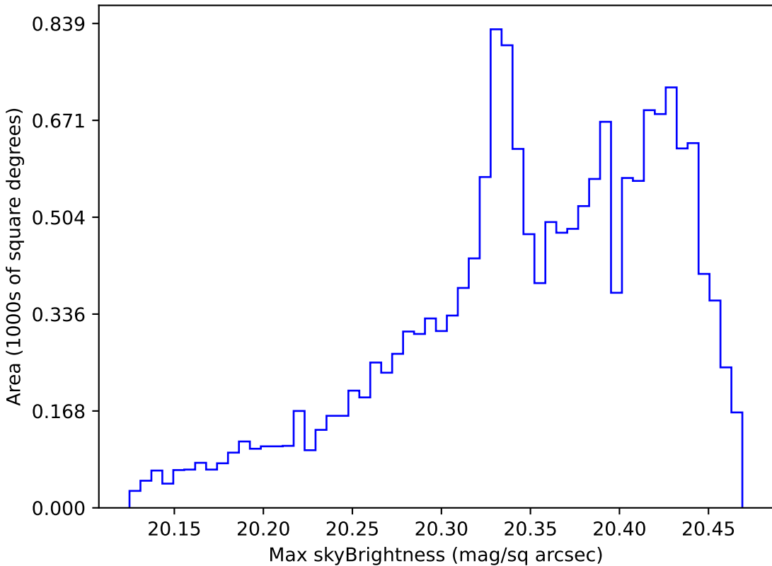
too_elab_r16_d2_griz_v3.4_10yrs WFD i band: Max skyBrightness
