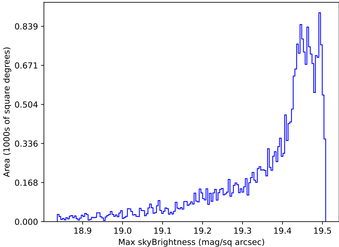
too_elab_r16_d2_griz_v3.4_10yrs All sky z band: Max skyBrightness
