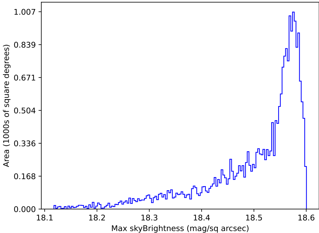
too_elab_r16_d2_griz_v3.4_10yrs All sky y band: Max skyBrightness
