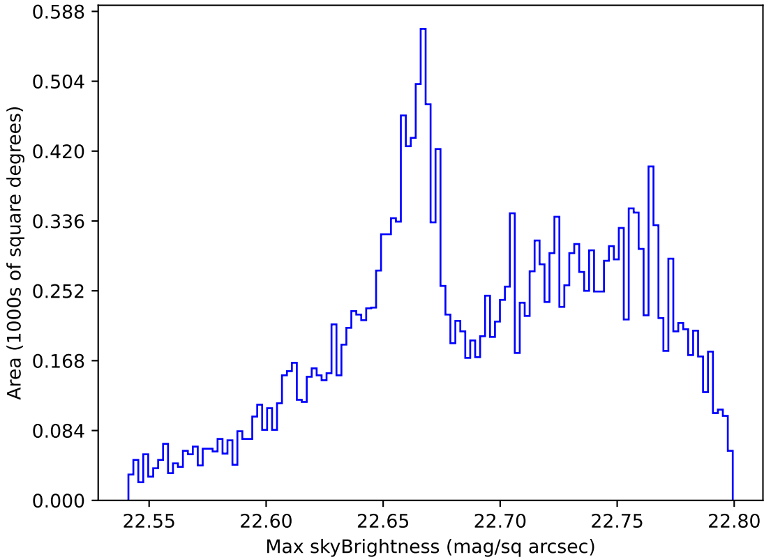
too_elab_r16_d2_griz_v3.4_10yrs All sky u band: Max skyBrightness
