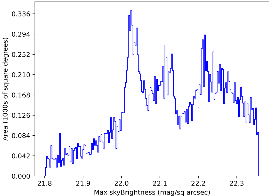
too_elab_r16_d2_griz_v3.4_10yrs All sky g band: Max skyBrightness
