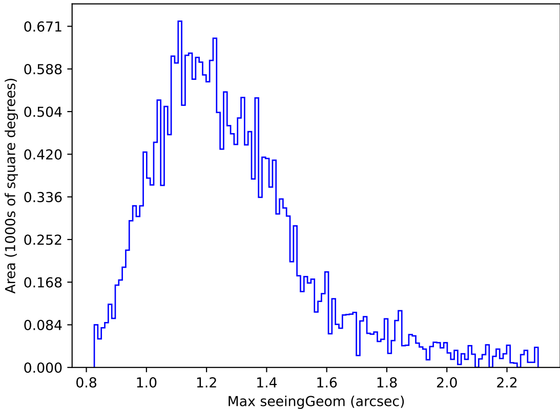
too_elab_r16_d2_griz_v3.4_10yrs Yr 1 z band: Max seeingGeom
