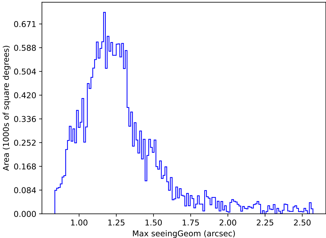
too_elab_r16_d2_griz_v3.4_10yrs Yr 1 y band: Max seeingGeom
