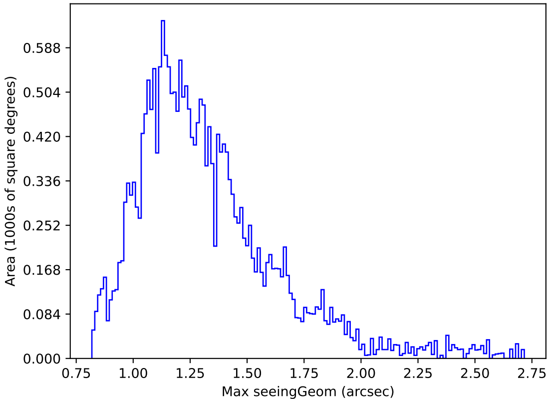
too_elab_r16_d2_griz_v3.4_10yrs Yr 1 u band: Max seeingGeom
