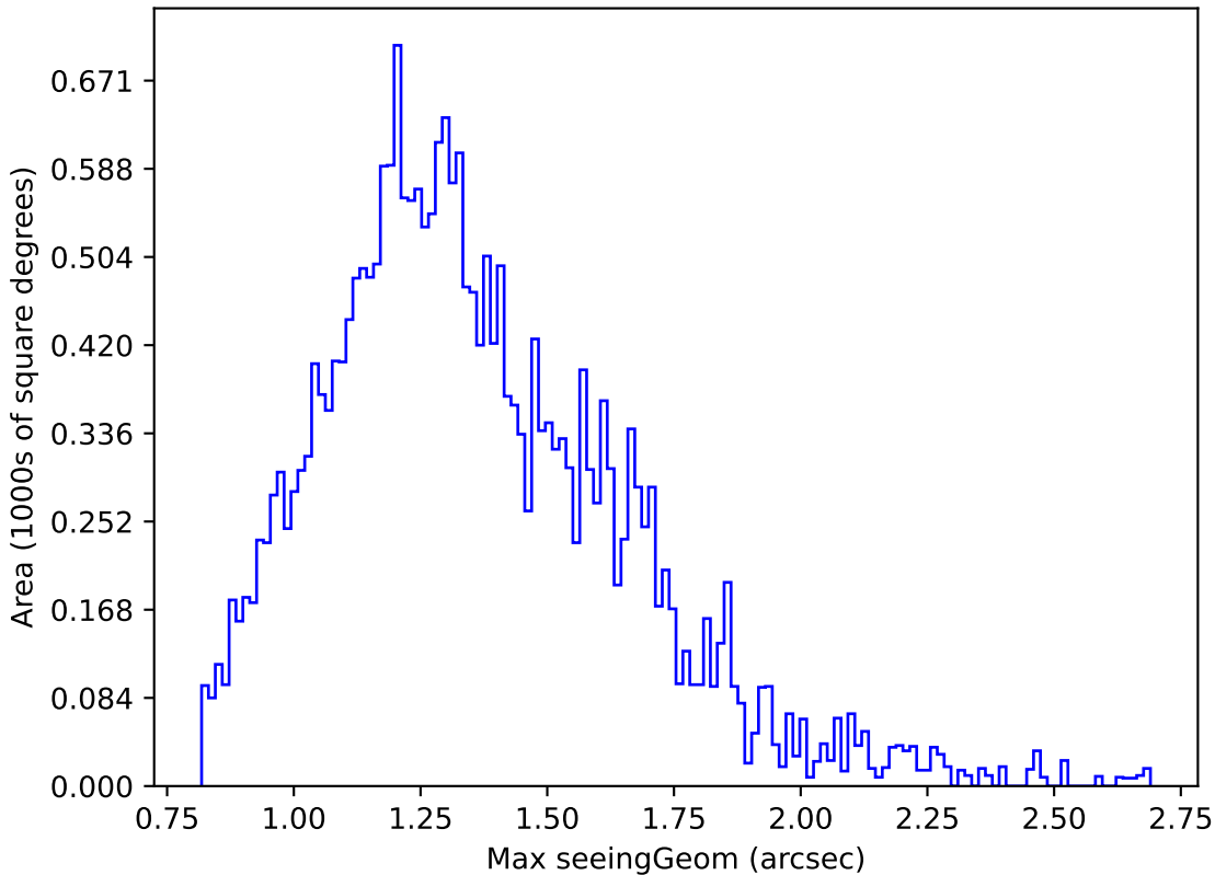
too_elab_r16_d2_griz_v3.4_10yrs Yr 1 r band: Max seeingGeom
