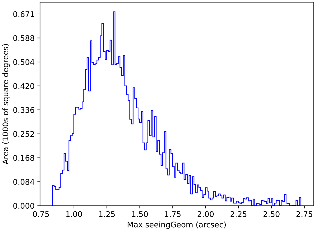
too_elab_r16_d2_griz_v3.4_10yrs Yr 1 i band: Max seeingGeom
