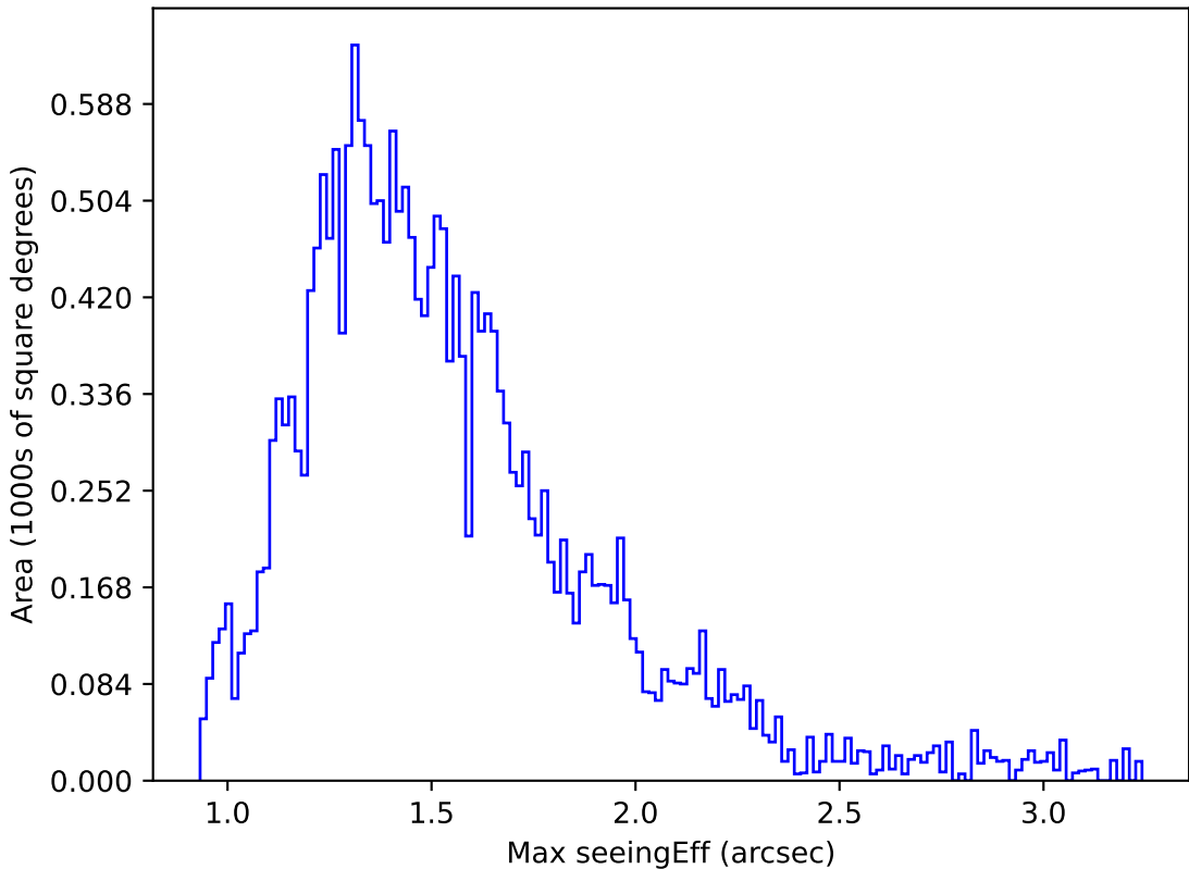
too_elab_r16_d2_griz_v3.4_10yrs Yr 1 u band: Max seeingEff
